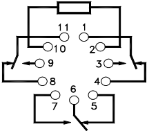
Wiring Diagram
