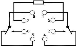
Wiring Diagram
